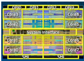
8/16 Cores Processor
