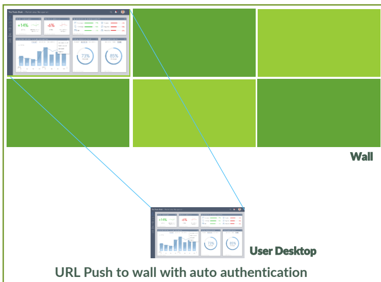
Soft KVM
